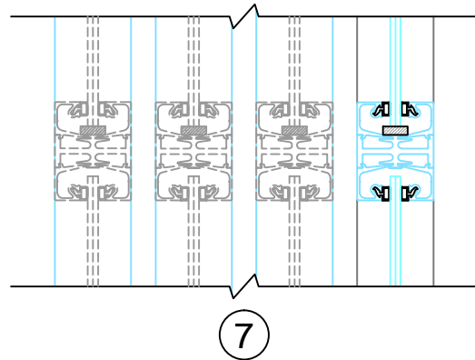
OPTIONAL MIDRAIL (VARIOUS SIZES AVAILABLE, VERTICAL OR HORIZONTAL)
